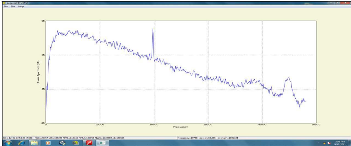
Fig.3. Receiving VLF signal from NWC station (freq: 19.8 KHz)
